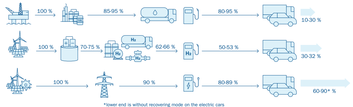
15 Illustration of energy losses for battery electric vehicle (EV), hydrogen fuel cell vehicle (HFCV) and internal combustion engine (ICE)
